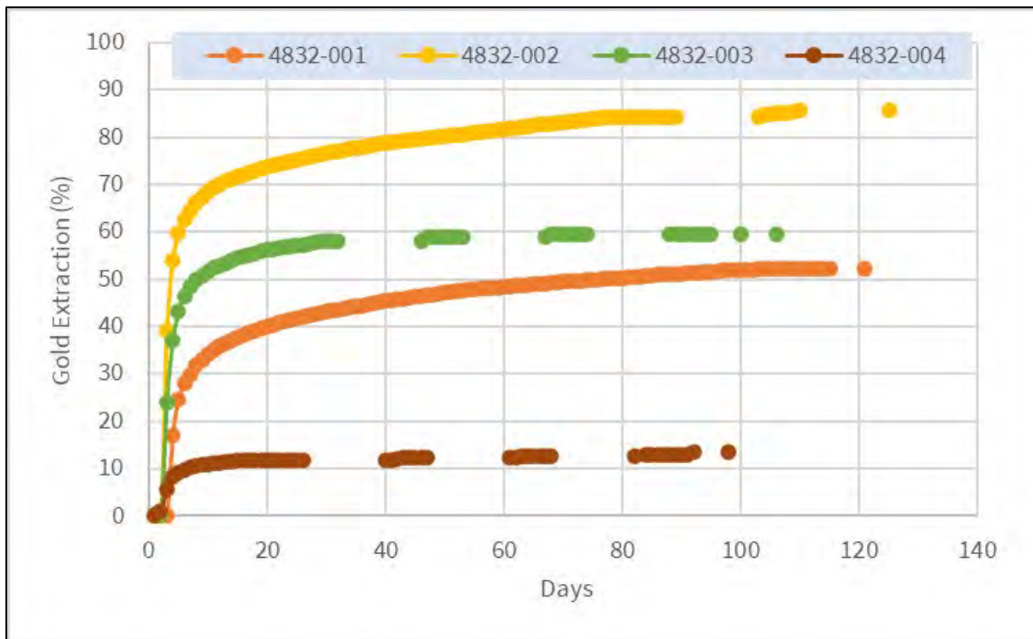
Figure 13.5 Column Leach Gold Recoveries - P 80 9.5 mm
