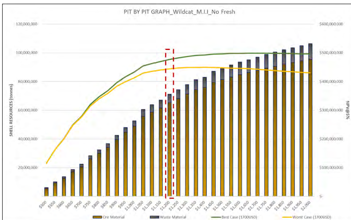
Figure 16.1 Wildcat Project Pit-by-Pit Graph
