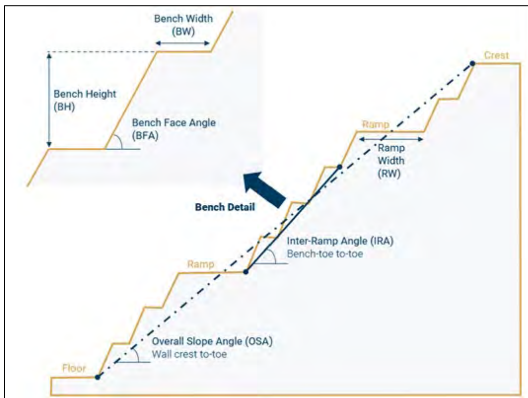
Figure 16.3 Pit Wall Terminology
