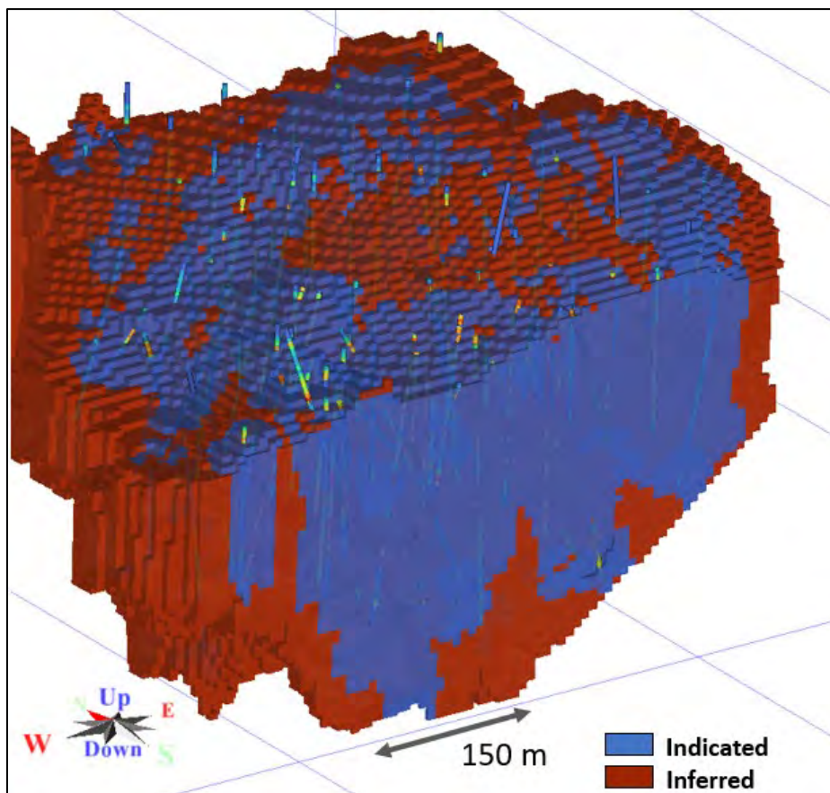
Figure 14.19 Mountain View Project 3D View of the Classification (Looking Northeast)
