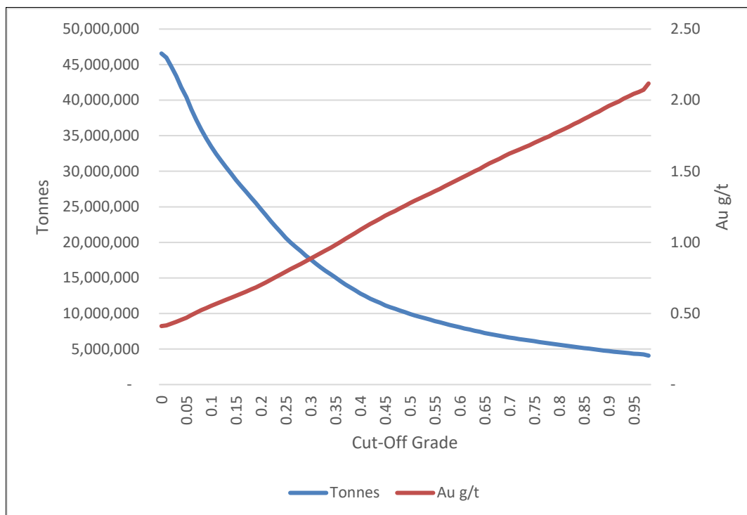
Figure 14.20 Mountain View Project, Grade Tonnage Curves for the Indicated Mineral Resources at Different Cut-Off Grades
