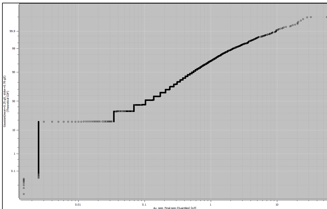
Figure 14.4 Wildcat Project, Logarithmic Probability Plots for Gold
