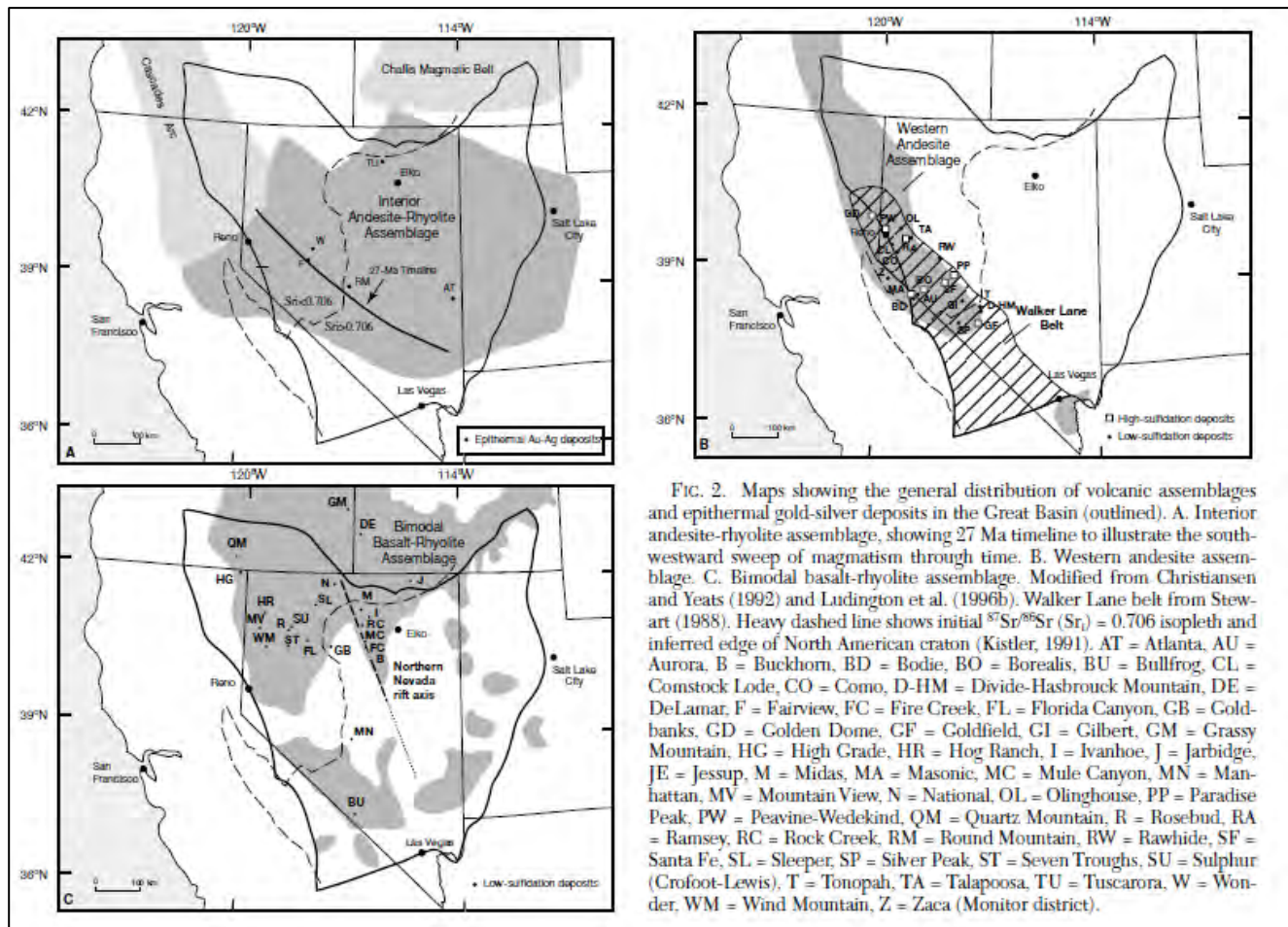
Figure 7.1 The Bimodal Basalt-Rhyolite Assemblage
