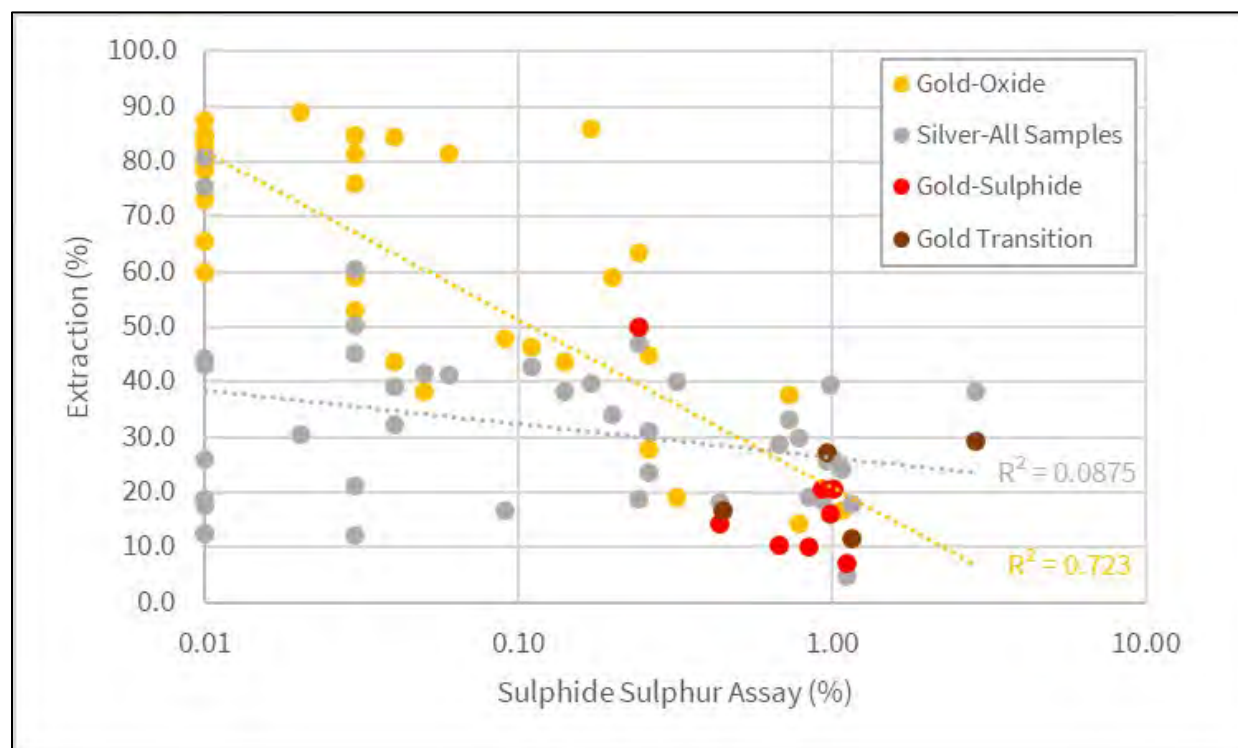
Figure 13.2 -1.7 mm Variability Bottle Roll Tests - Au and Ag Recovery versus Sulphide Sulphur Content
