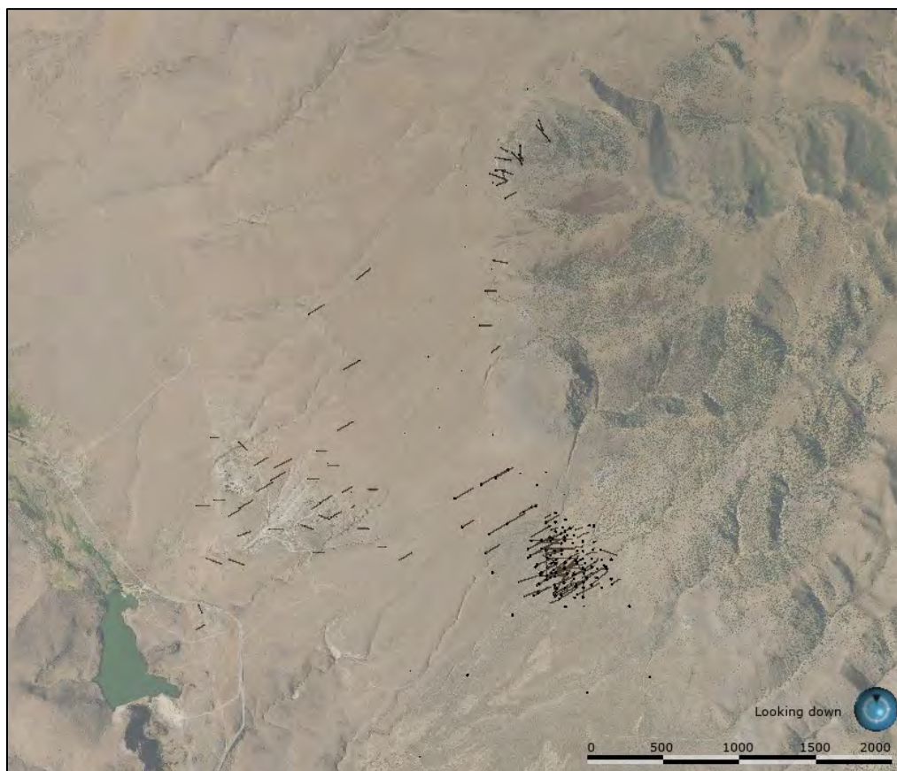
Figure 14.12 Mountain View Project, Plan View of Drilling Locations
