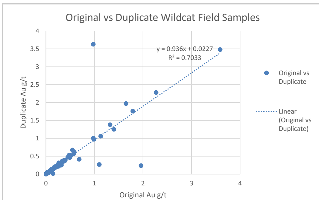
Figure 11.3 Graph of Field Duplicate Performance at the Wildcat Project
