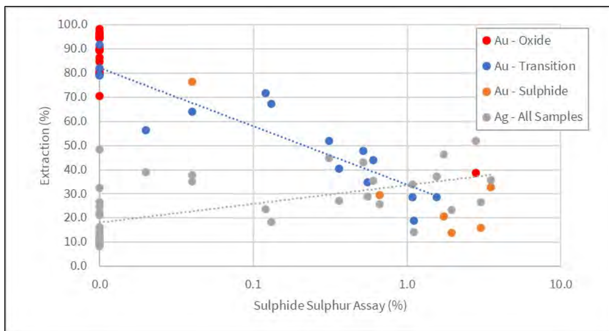
Figure 13.8 -1.7 mm Variability Bottle Roll Tests - Au and Ag Recovery versus Sulphide Sulphur Content
