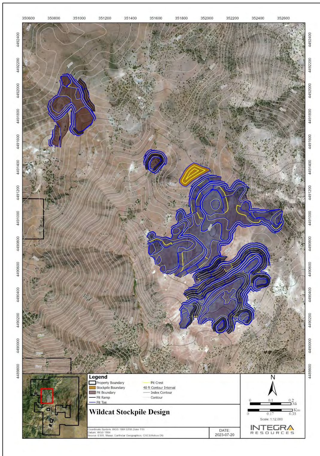
Figure 16.13 Wildcat Project, Mineralized Material Stockpile Design
