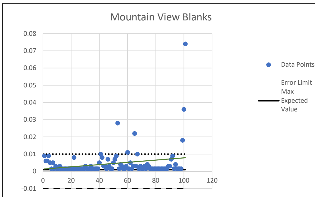
Figure 11.5 Graph of Blank Performance at Mountain View Project
