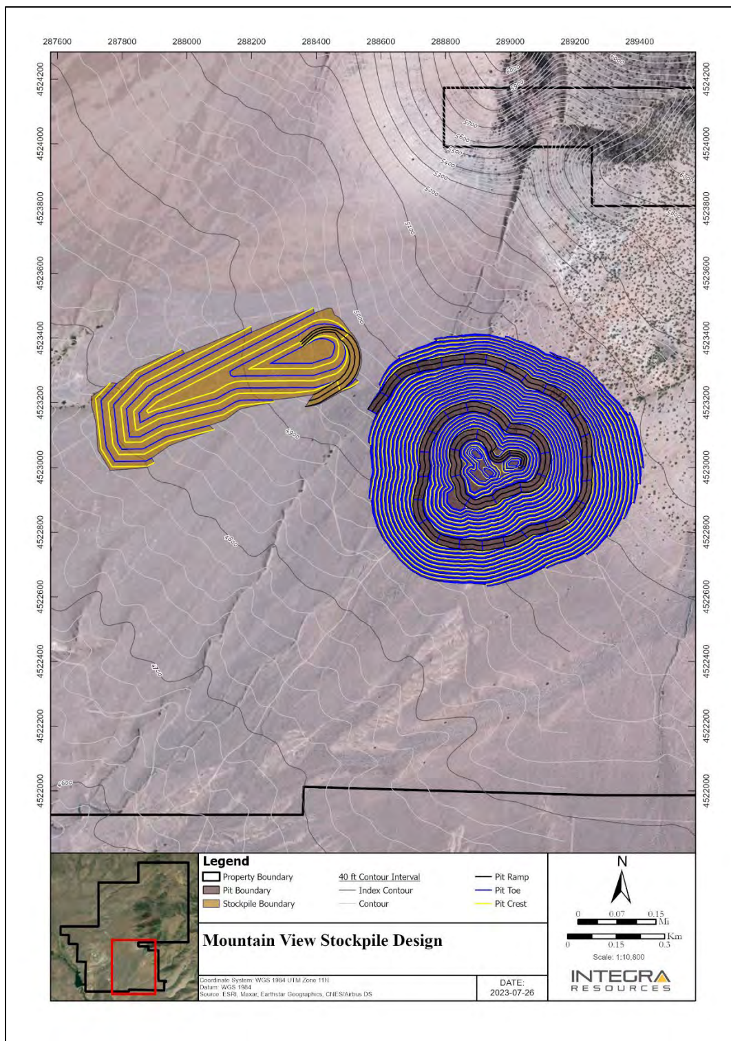
Figure 16.14 Mountain View Project, Mineralized Material Stockpile Design
