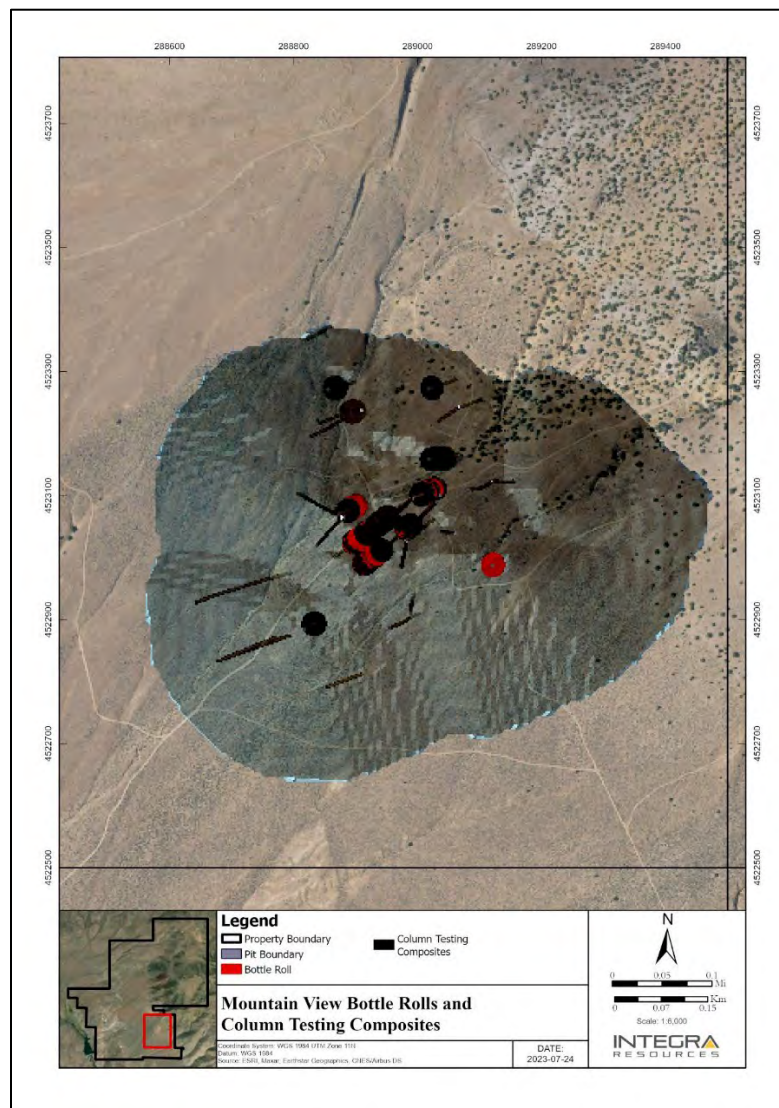
Figure 13.7 Mountain View Metallurgical Samples Locations
