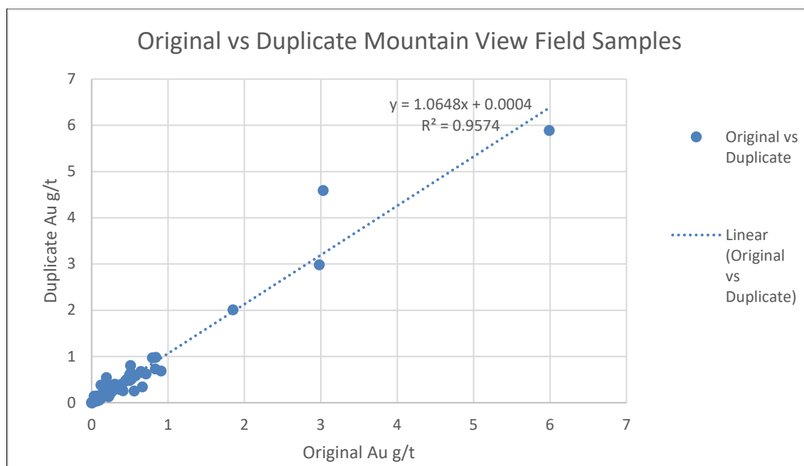
Figure 11.6 Graph of Duplicate Performance at Mountain View Project
