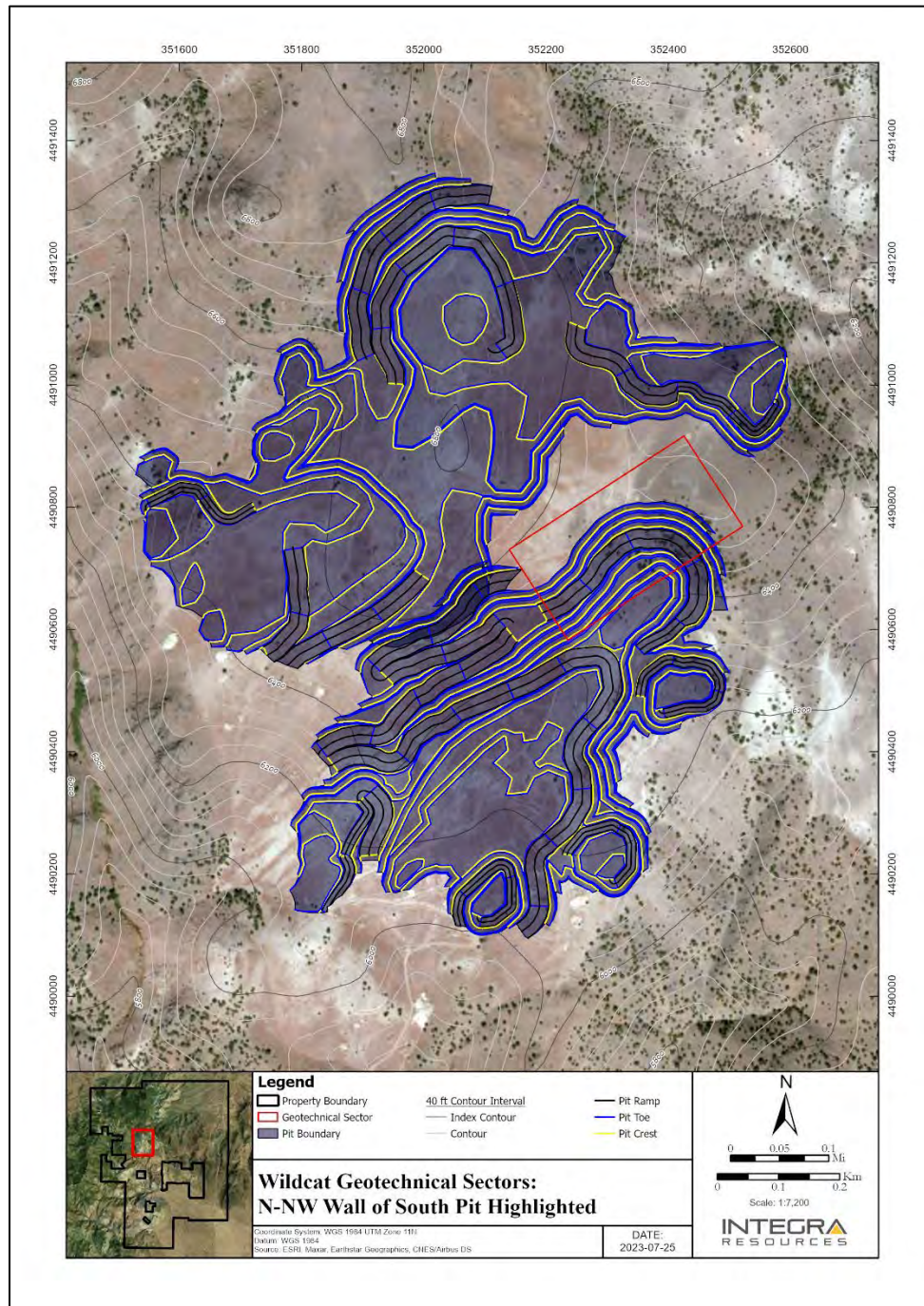
Figure 16.4 Wildcat Geotechnical Sectors: North-Northwest Wall of South Pit Highlighted
