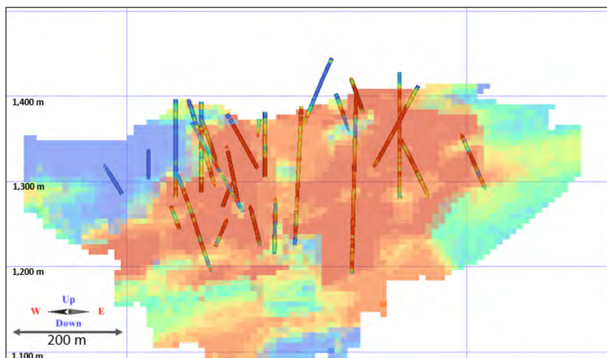
Figure 14.17 Mountain View Project, North-South Block Model Cross Section Visual Checks (Looking North)
