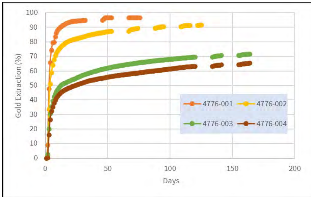
Figure 13.13 Mountain View Project, Column Leach Gold Recoveries – P 80 9.5 mm
