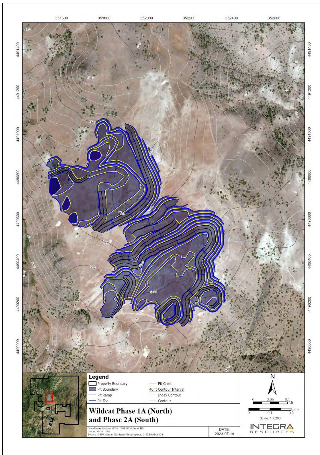
Figure 16.5 Wildcat Pit, Phase 1A (North) and Phase 2A (South)
