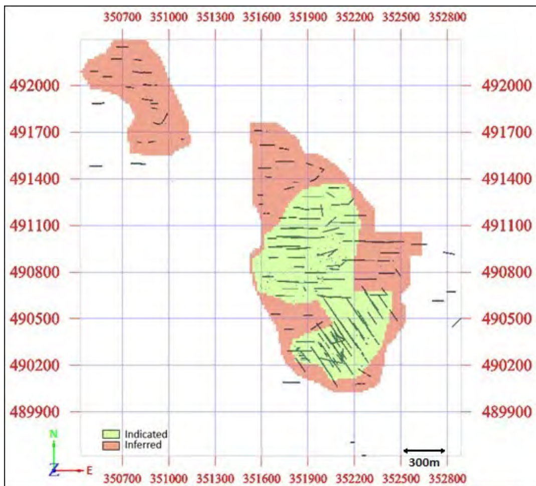
Figure 14.9 Wildcat Project, Plan View of the Mineral Resource Classification
