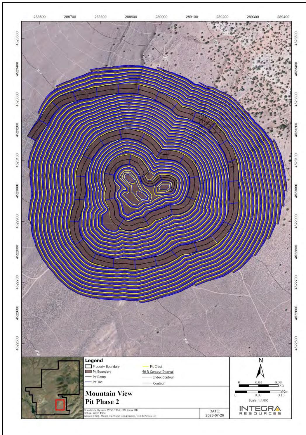
Figure 16.10 Mountain View Final Pit Phase 2
