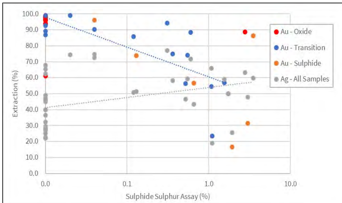
Figure 13.10 P 80 75 µm Variability Bottle Roll Tests - Au and Ag Recovery versus Sulphide Sulphur Content
