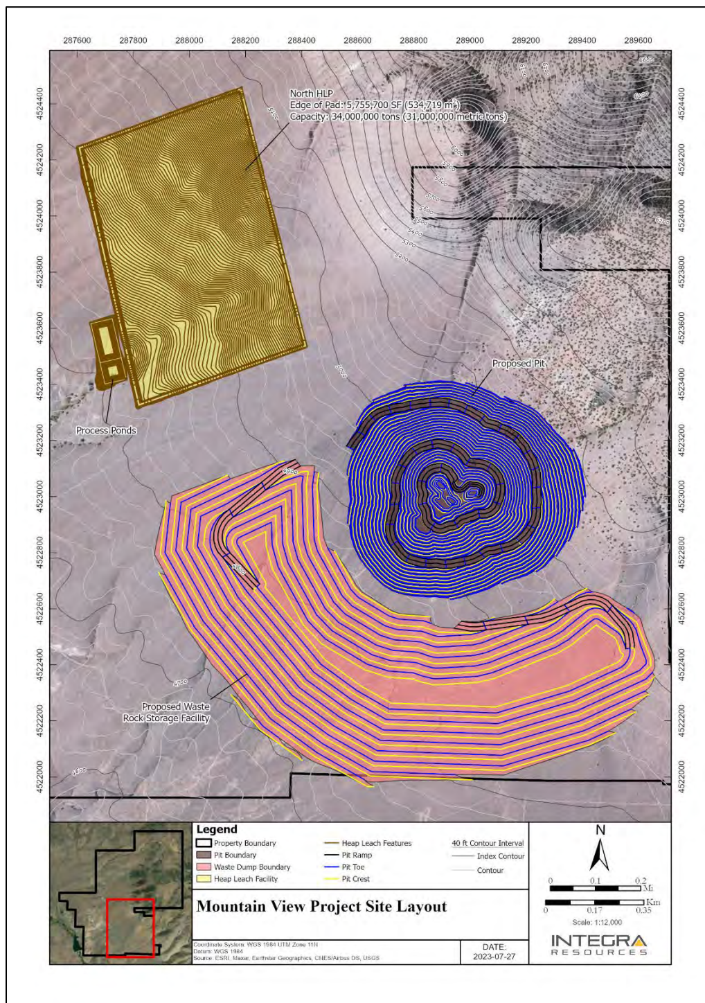
Figure 18.2 Mountain View Project Site Layout
