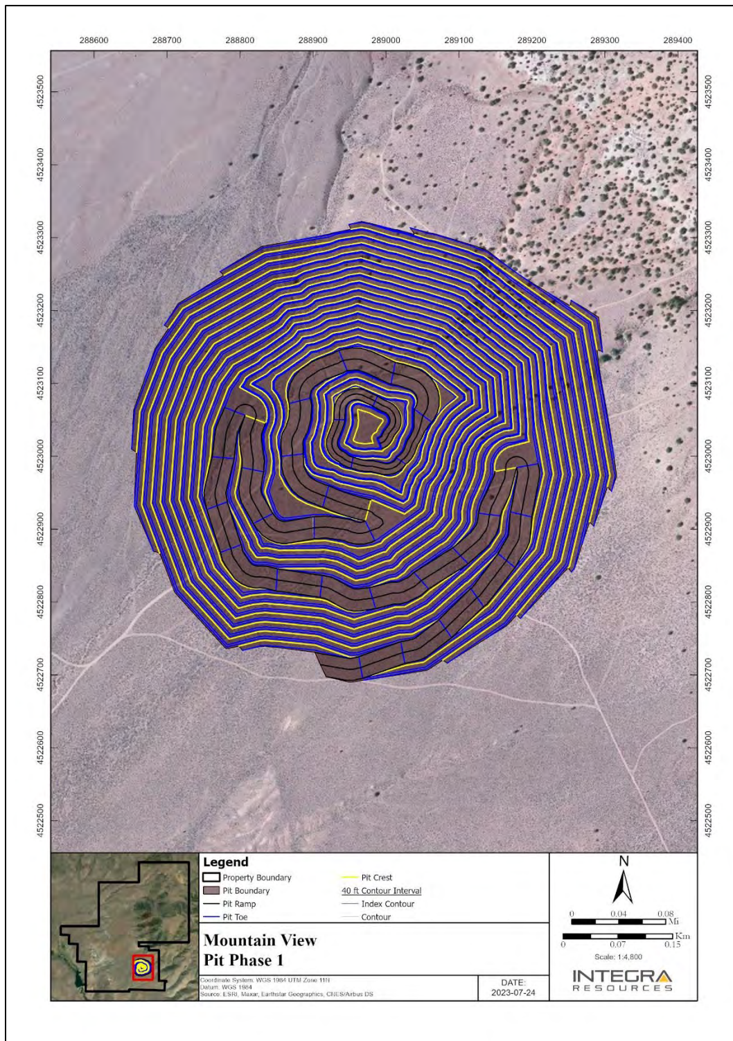
Figure 16.9 Mountain View Pit Phase 1
