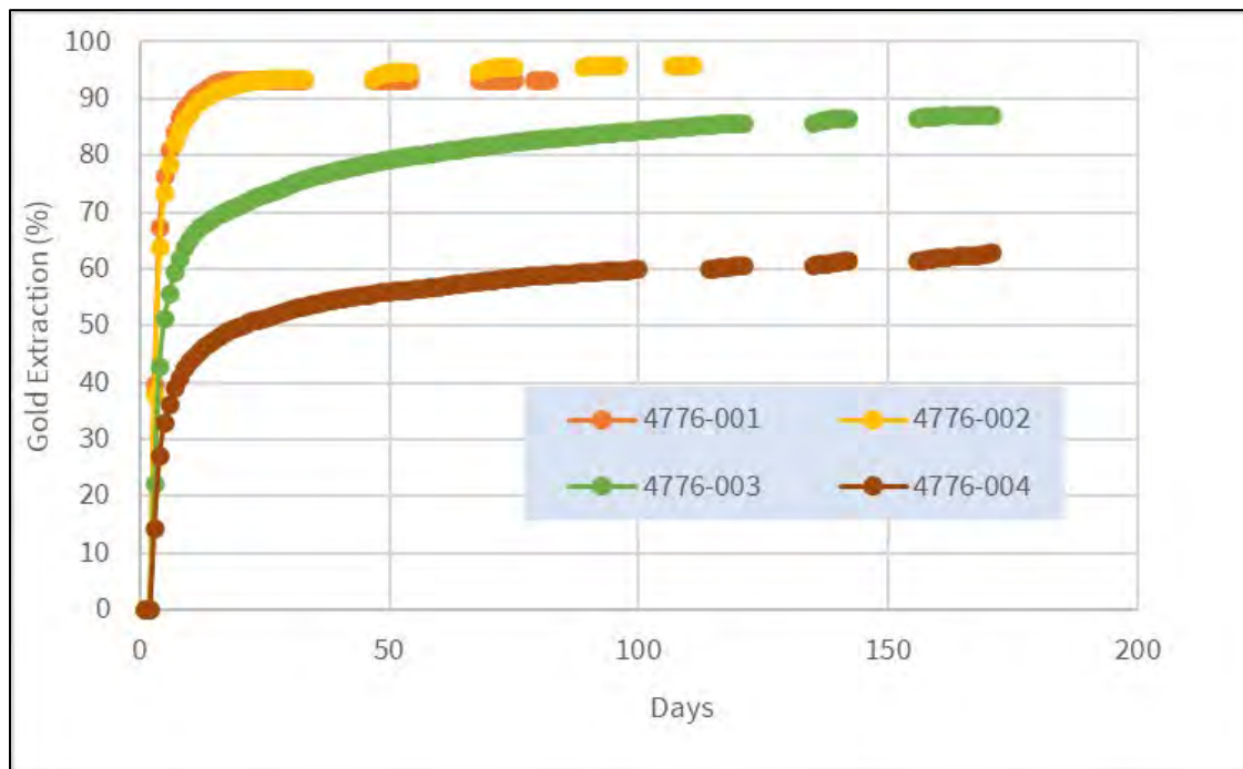
Figure 13.13 Mountain View Project, Column Leach Gold Recoveries – P 80 9.5 mm
