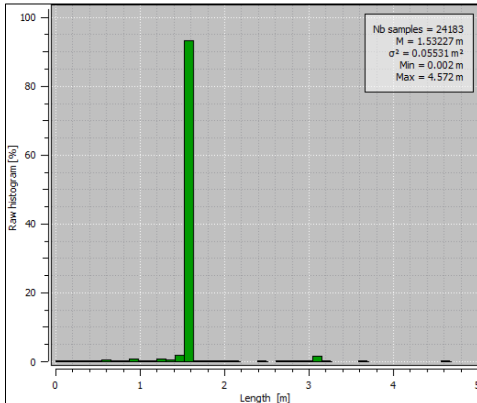
Figure 14.6 Wildcat Project, Assays Length Histogram
