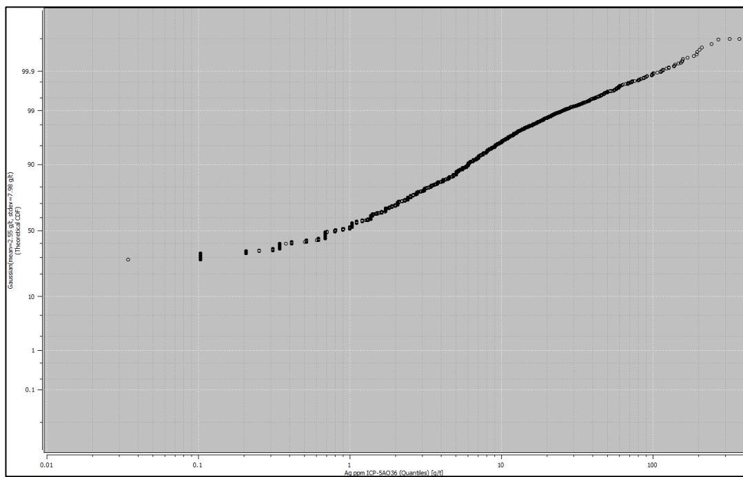
Figure 14.5 Wildcat Project, Logarithmic Probability Plots for Silver
