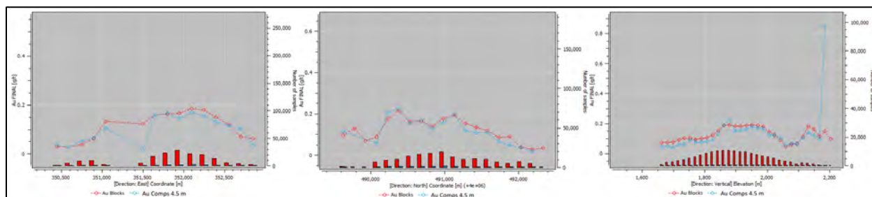
Figure 14.8 Wildcat Project, Gold Trend Plot: East, North and Elevation
