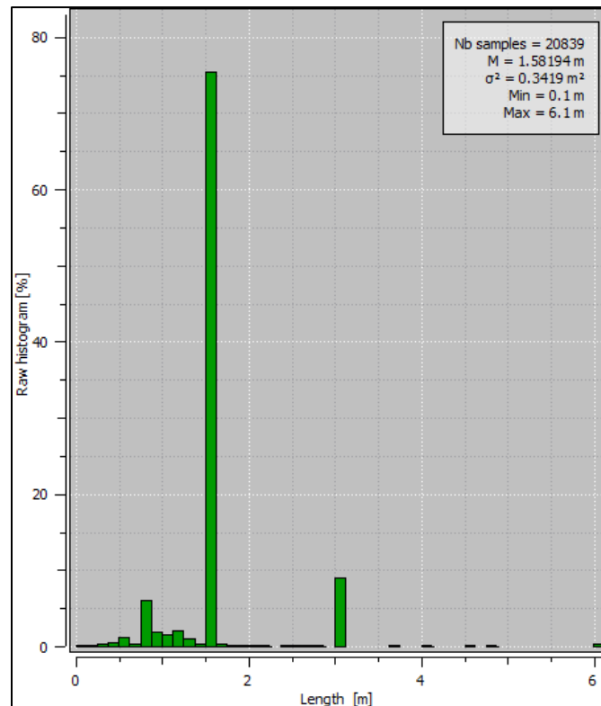
Figure 14.16 Mountain View Project, Assay Length Histogram
