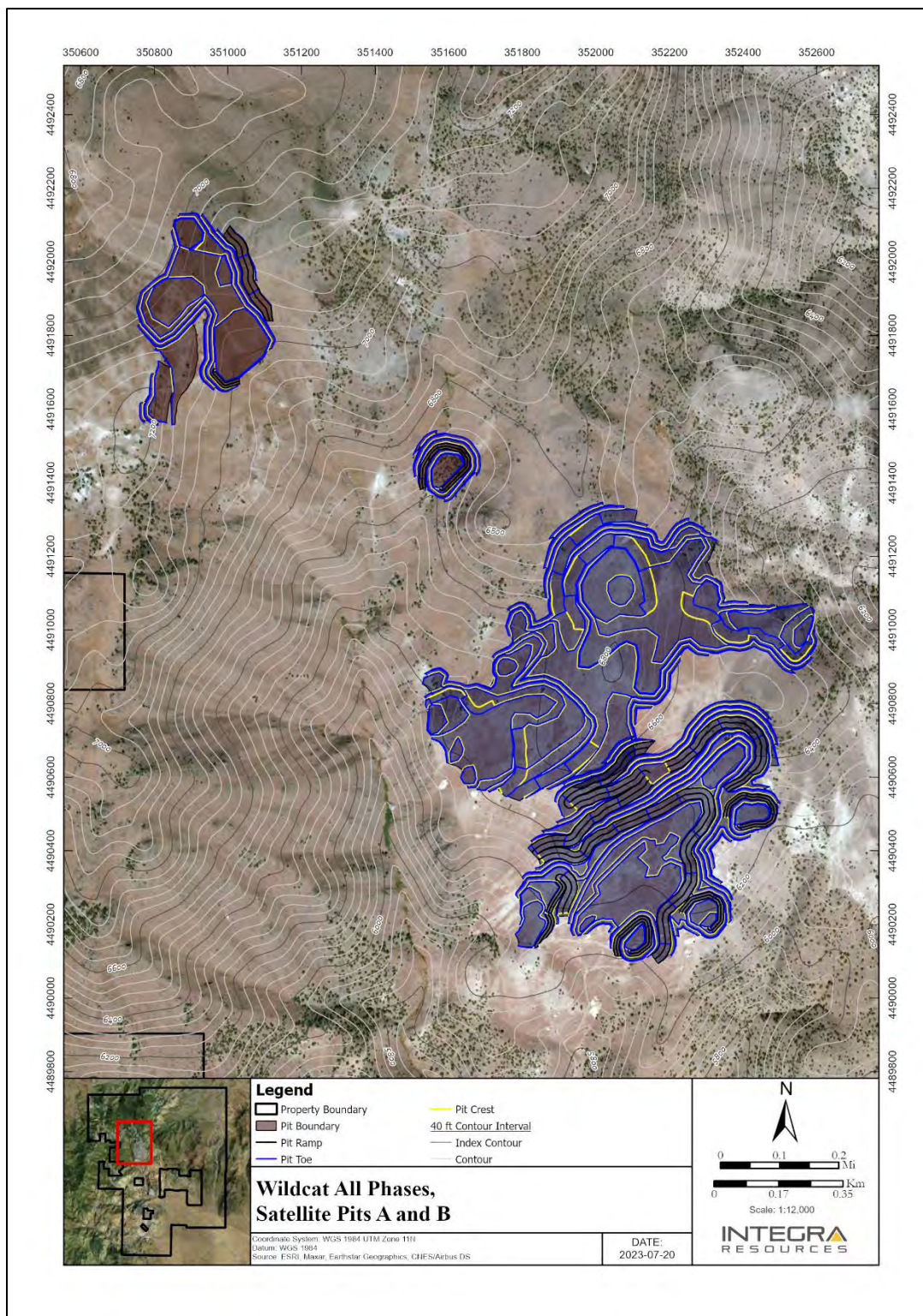
Figure 16.8 Wildcat Pit all Phases, Satellite Pits A and B
