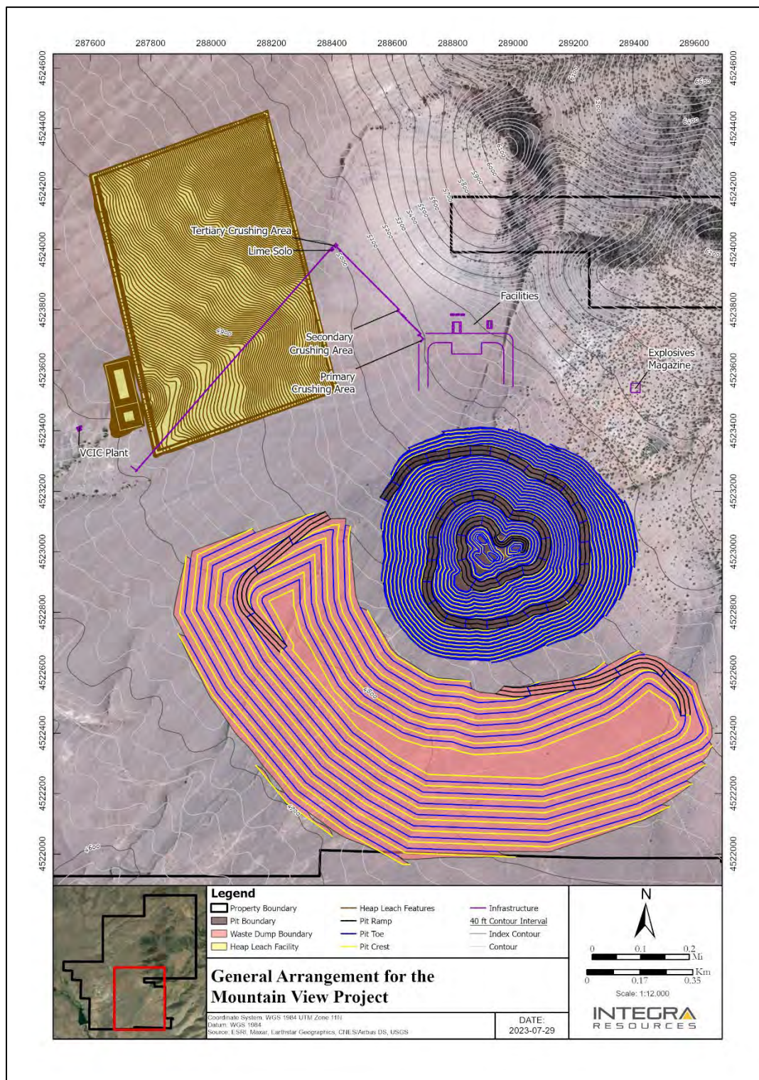
Figure 18.4 General Arrangement for the Mountain View Project
