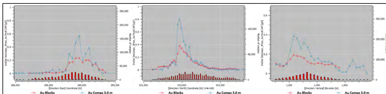
Figure 14.18 Mountain View Project, Gold Trend Plot for East, North and Elevation
