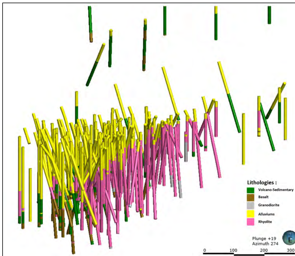
Figure 14.13 Mountain View Project, 3D View of the Drilling Lithologies at the Main Hill Zone (Looking West)
