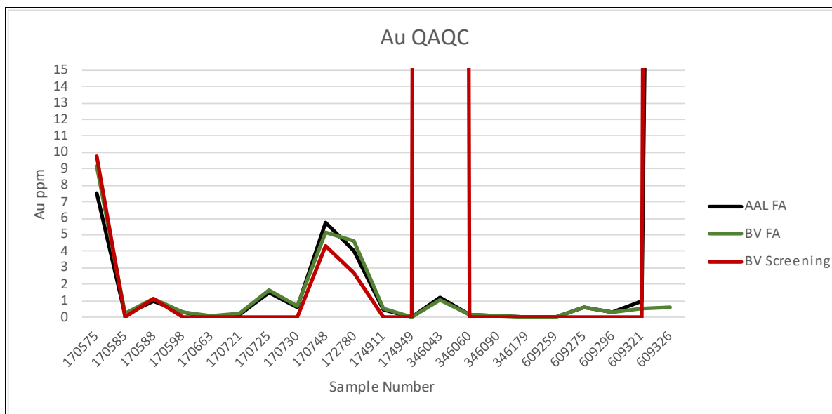
Figure 12.8 Comparison between the Original Assay from AAL and the Bureau Veritas Check Re-Assays
