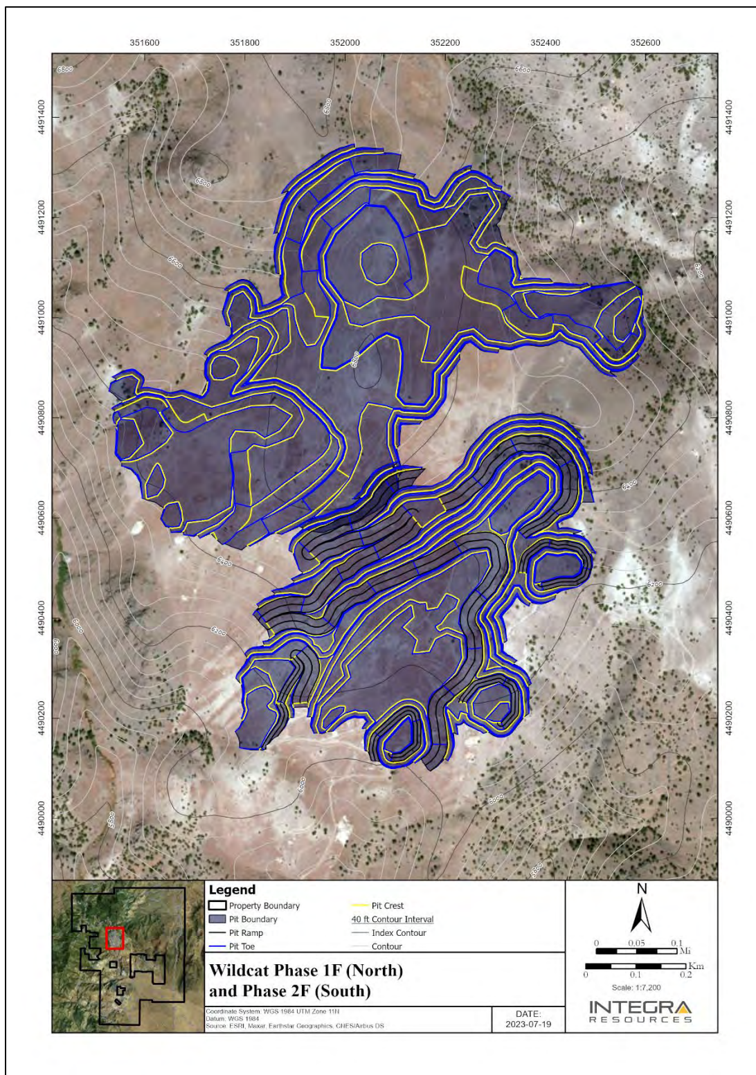
Figure 16.6 Wildcat Pit, Phase 1F (North) and Phase 2F (South)
