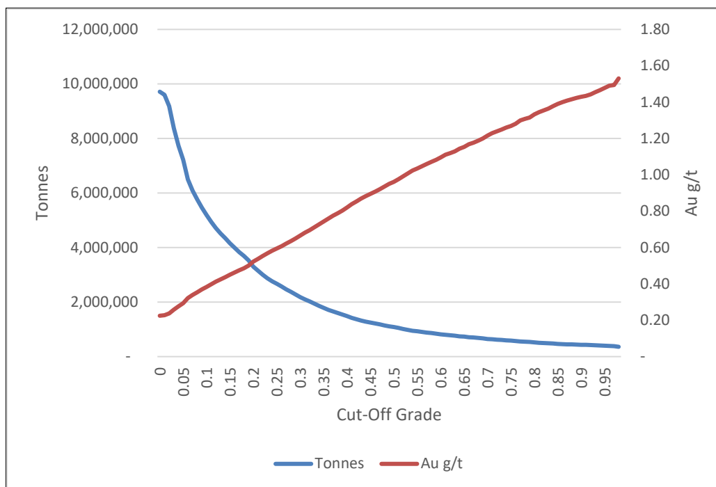
Figure 14.21 Mountain View Project, Grade Tonnage Curves for the Inferred Mineral Resources at Different Cut-Off Grades
