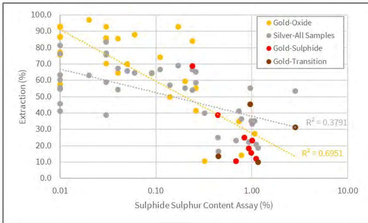
Figure 13.3 P 80 75 µm Variability Bottle Roll Tests - Au and Ag Recovery versus Sulphide Sulphur Content
