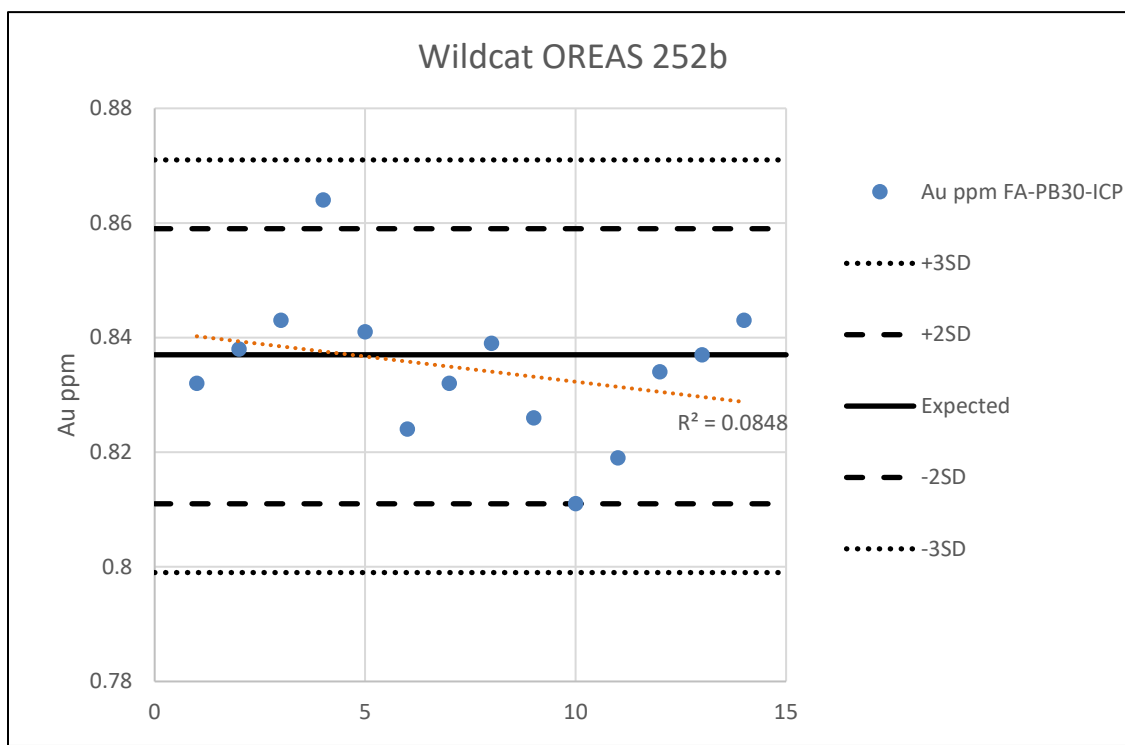
Figure 11.1 Example of AAL Results for Standard OREAS 252b for the Wildcat 2022 Drill Program
