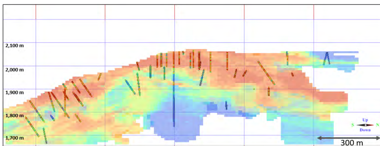
Figure 14.7 Wildcat Project, North-South Block Model Cross Section Visual Checks (Looking West)
