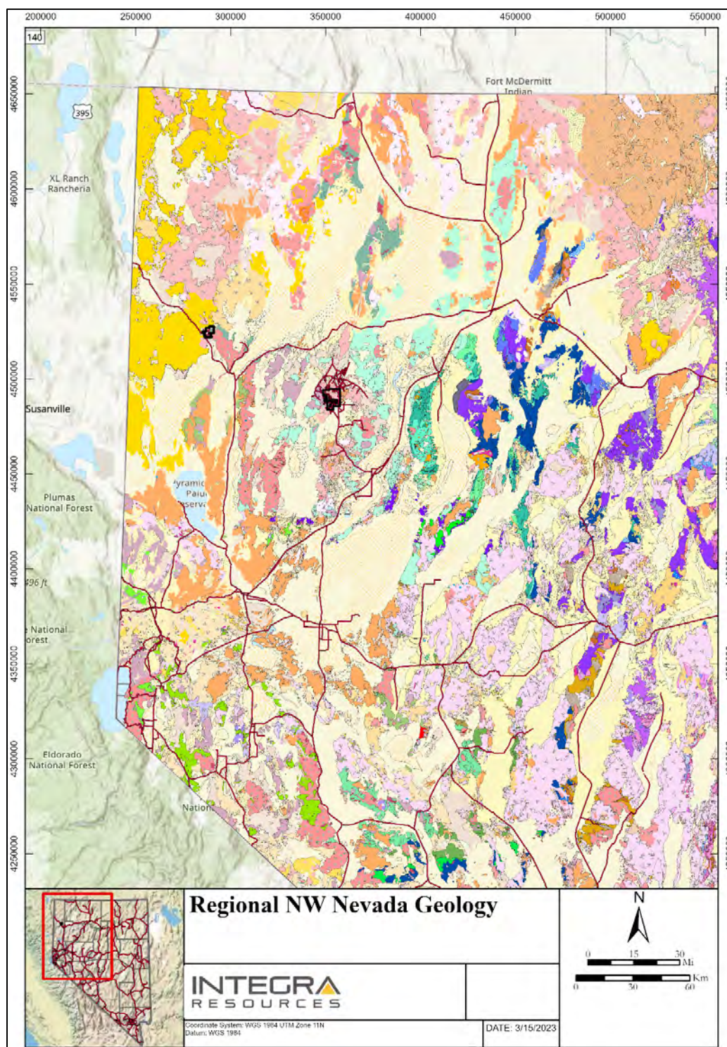
Figure 7.3 Regional Geology Map for Northwest Nevada
