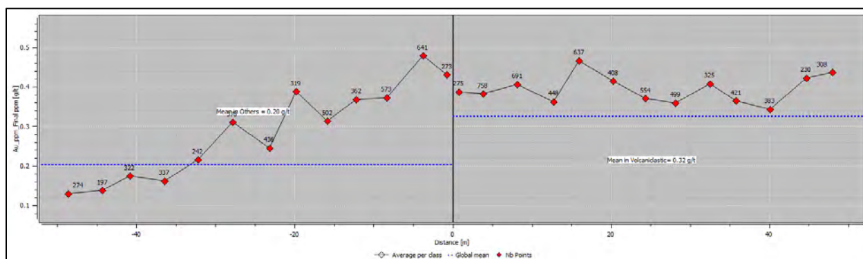
Figure 14.3 Wildcat Project, Volcanoclastic Contact Plot
