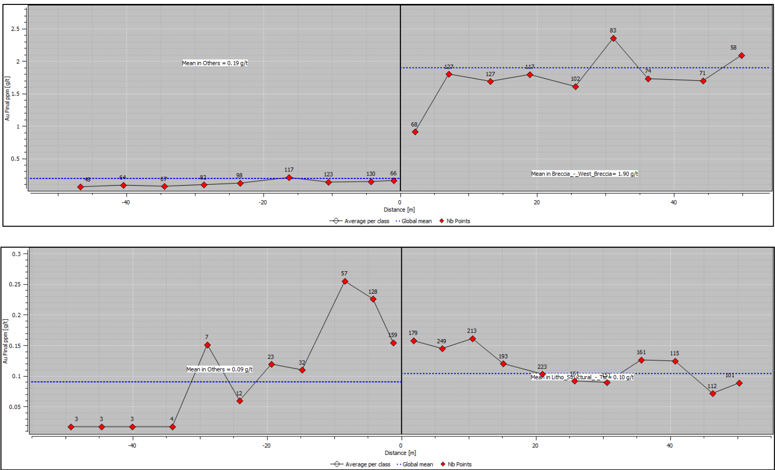
Figure 14.14 Mountain View Project, West Breccia and Rhyolite Contact Plots
