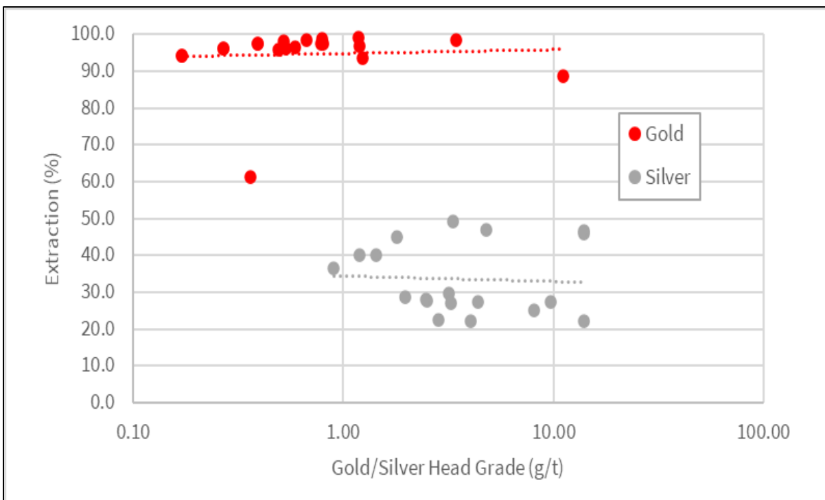
Figure 13.11 P 80 75 µm Oxide Variability Bottle Roll Tests - Au and Ag Extraction versus Head Grade
