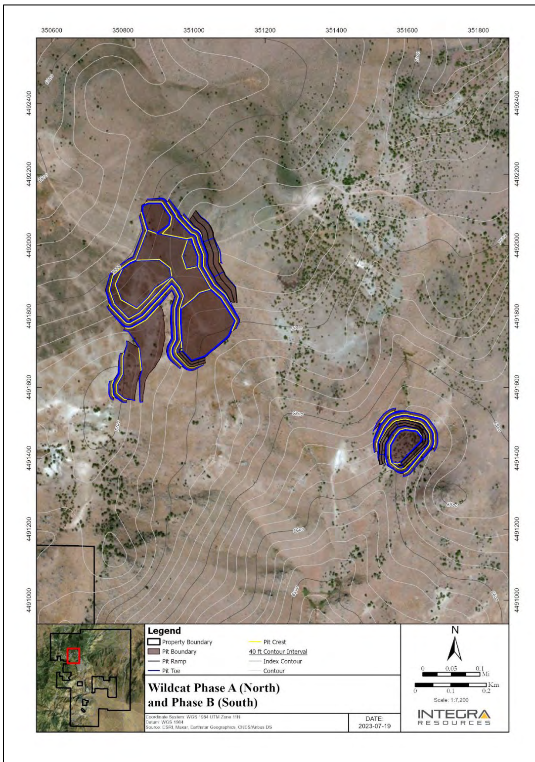
Figure 16.7 Wildcat Pit, Phase A (North) and Phase B (South)
