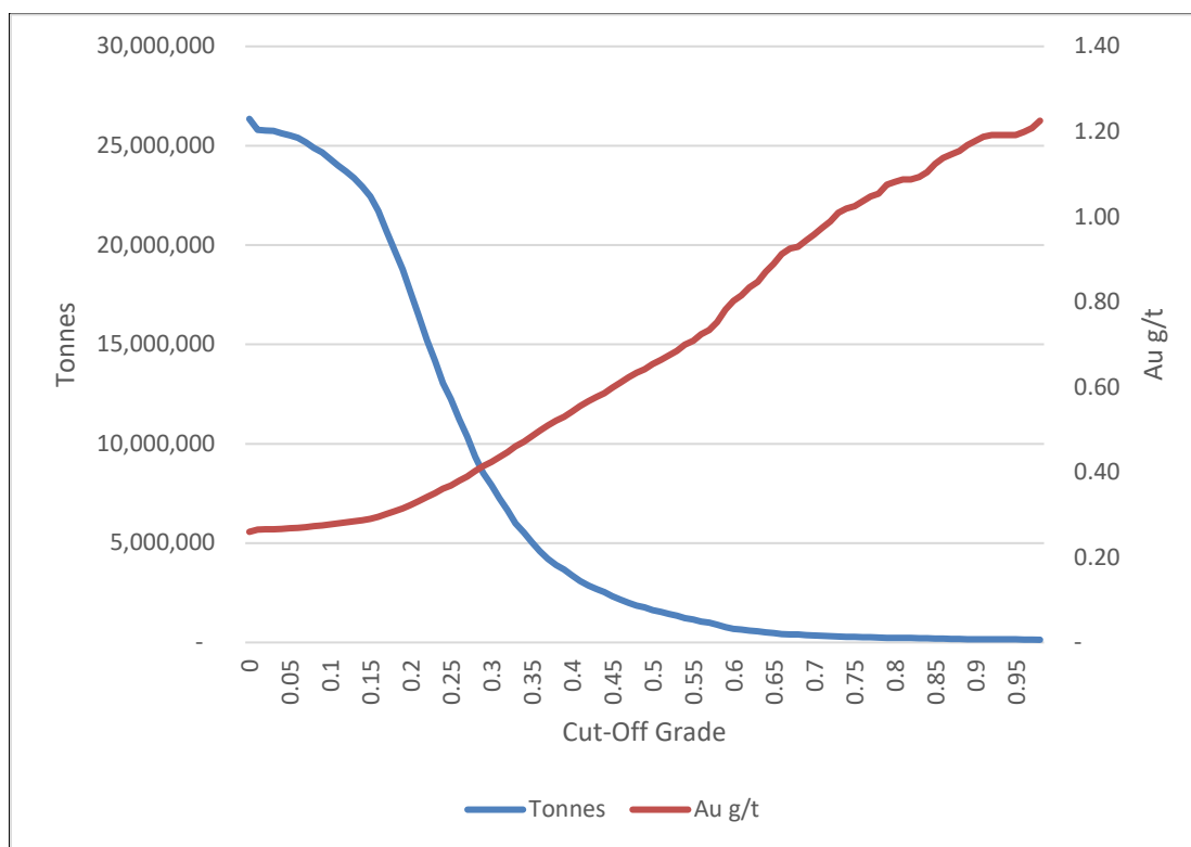
Figure 14.11 Wildcat Project, Grade Tonnage Curves for the Inferred Mineral Resources at Different Cut-Off Grades
