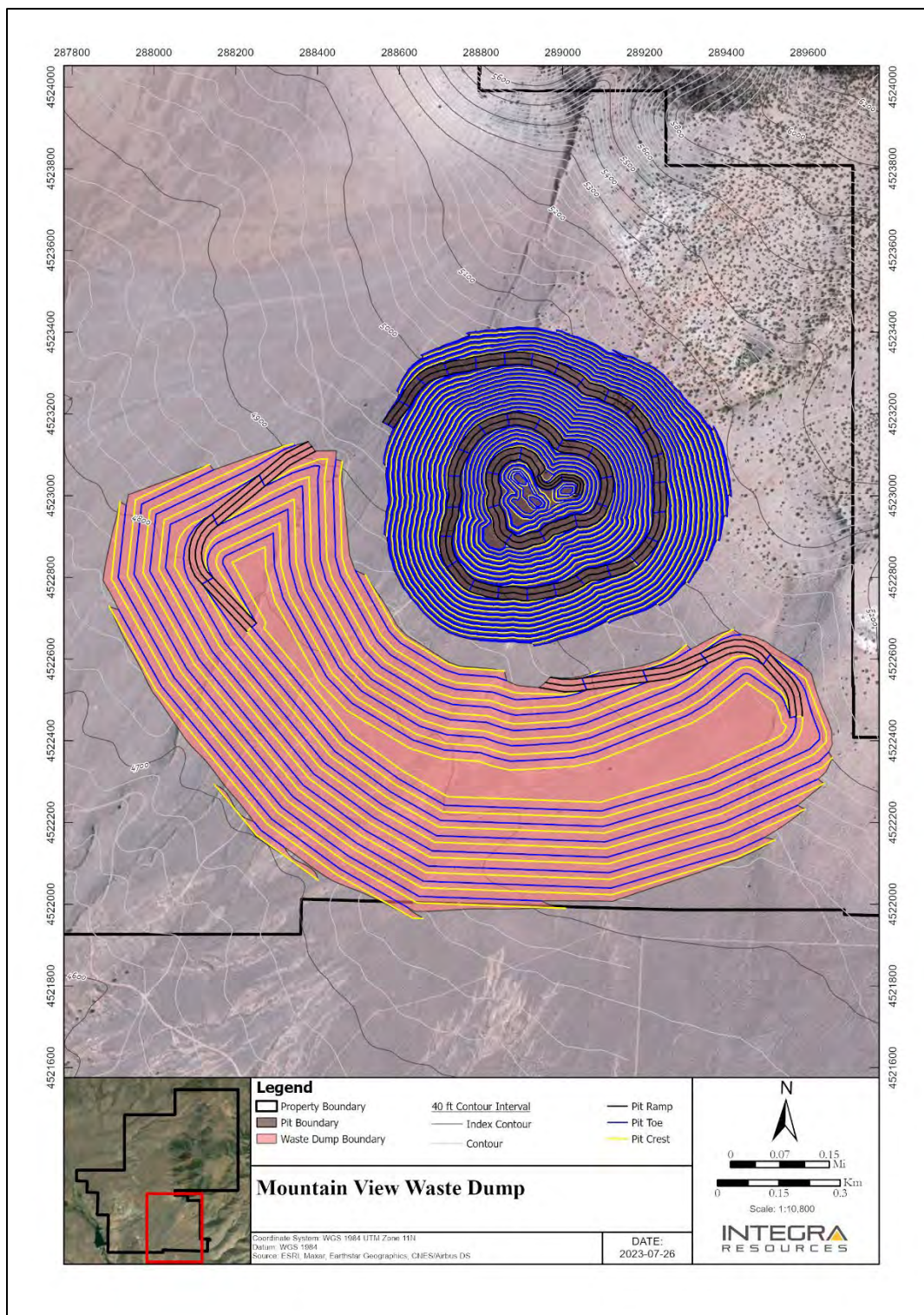
Figure 16.12 Mountain View Project, Waste Dump
