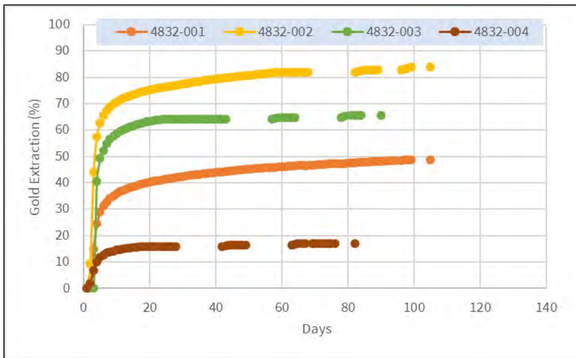
Figure 13.6 Column Leach Gold Recoveries – P 80 6.3 mm (HPGR)
